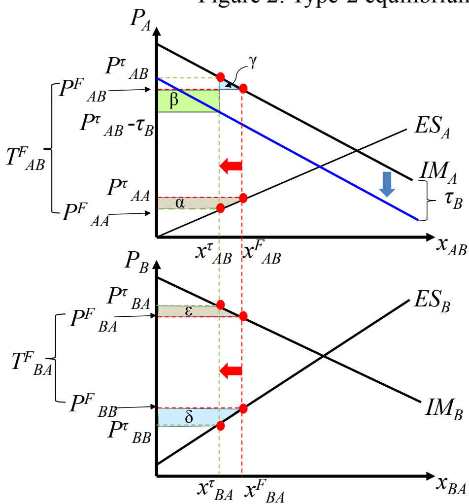
Figure 2: Type-2 equilibrium
